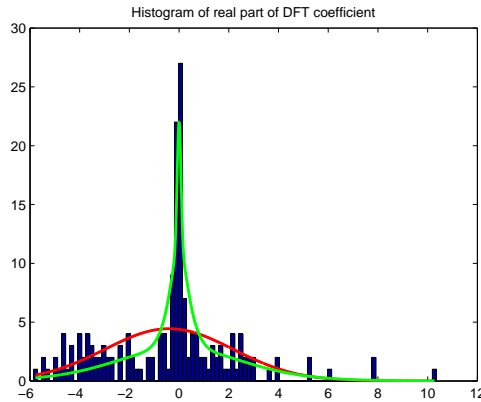
Figure 2.11: Gaussian mixture model for DFT coefficients.
