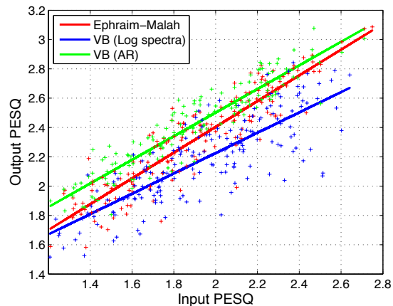
Figure 3: Comparison of perceptual quality performance.
