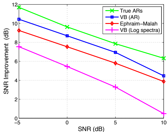
Figure 1: SNR improvement versus input SNR.
