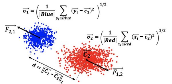
Fig. 2. Definition of parameters in a model with two classes in which G is gravitization constant, \vec{\sigma}_1 and \vec{\sigma}_2 are the standard deviation of class 1 and class 2 respectively, d is the L_2 norm distance between two centroids c_1 and c_2 which are associated to class 1 and class 2 respectively
